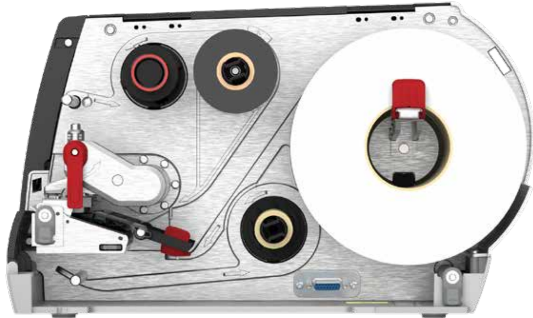
Fixed Media Hanger + Label Roll Core 76 mm (3.0 in) ID Shown with Label Roll 213 mm (8.38 in) OD Typical length of material with typical thickness of labels ~ 195 m
